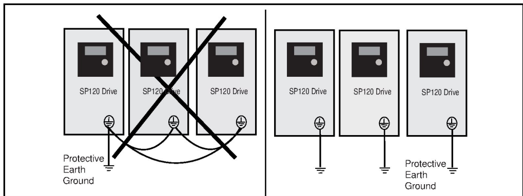
Figure 2.5 – Grounding the Drive
