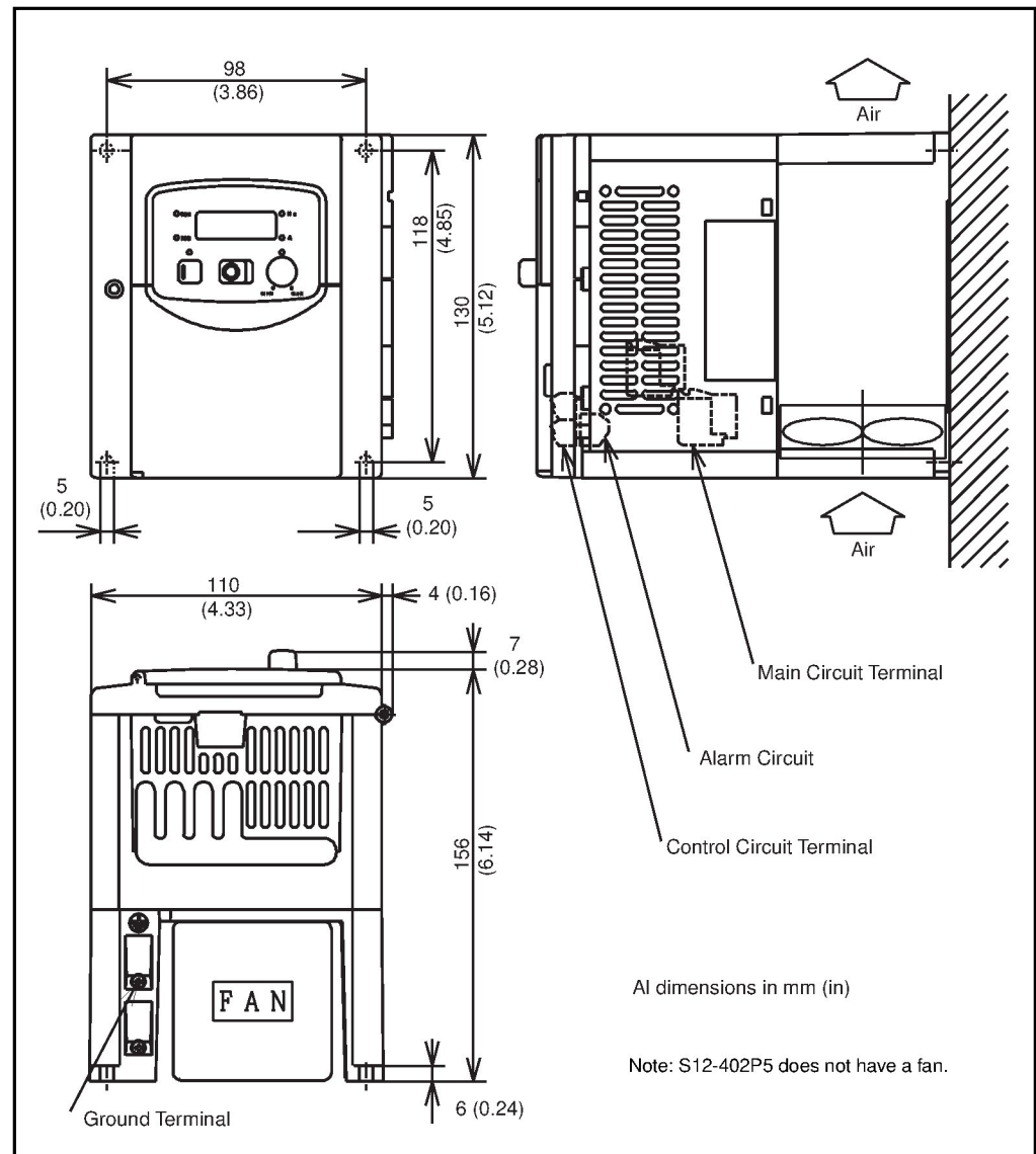
Figure A.7 – S12-402P5/403P8/405P5 Dimensions
