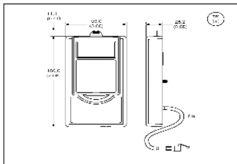
Figure 2 - Bezel Dimensions
