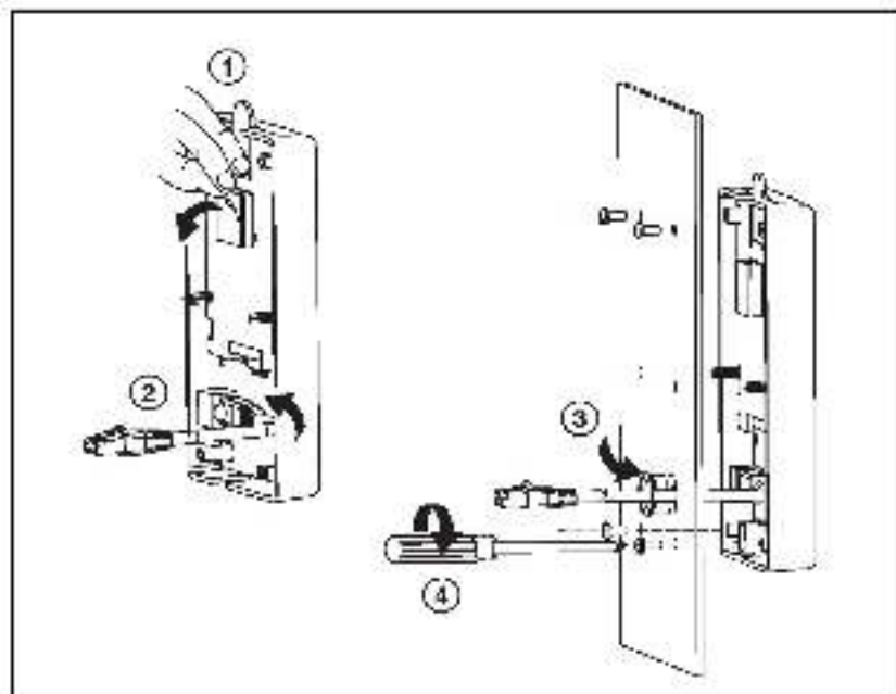
Figure 5 – Mounting the Bezel
