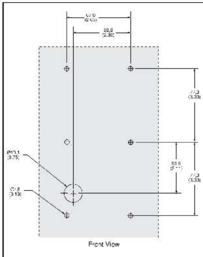
Figure 4 – Mounting Template (Not Actual Size)
