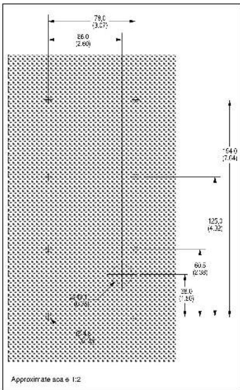
Figure 3 – Mounting template
