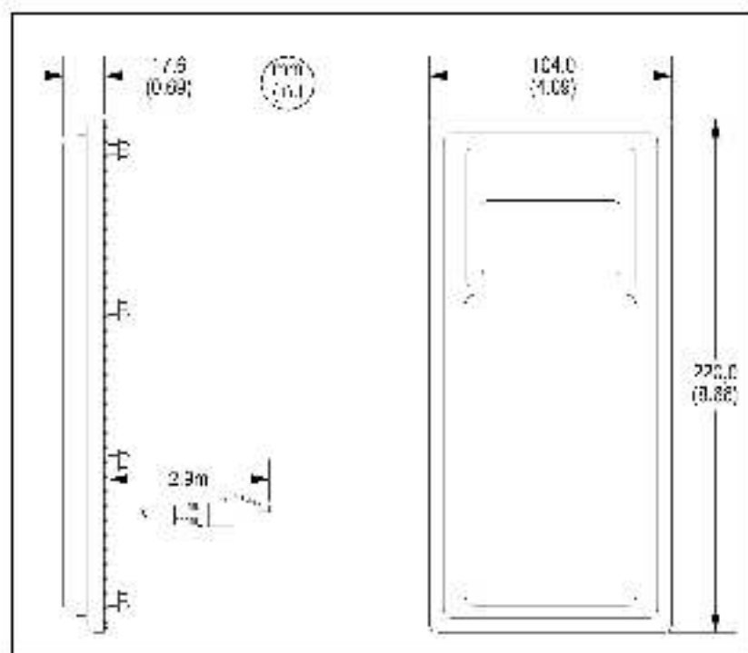
Figure 2 — MO50 Remote CIM Dimensions
