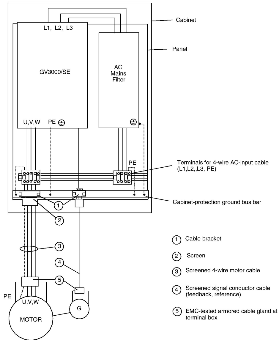
Figure C.4 – Cabinet-Mounted GV3000/SE Wiring Example
