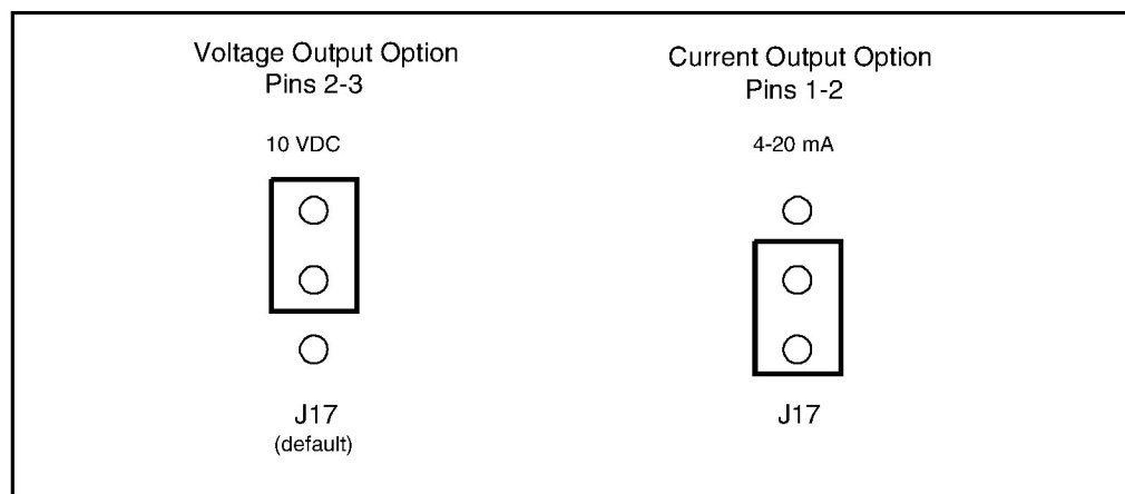
Figure 2.13 – Jumper J17 Settings for Analog Outputs
