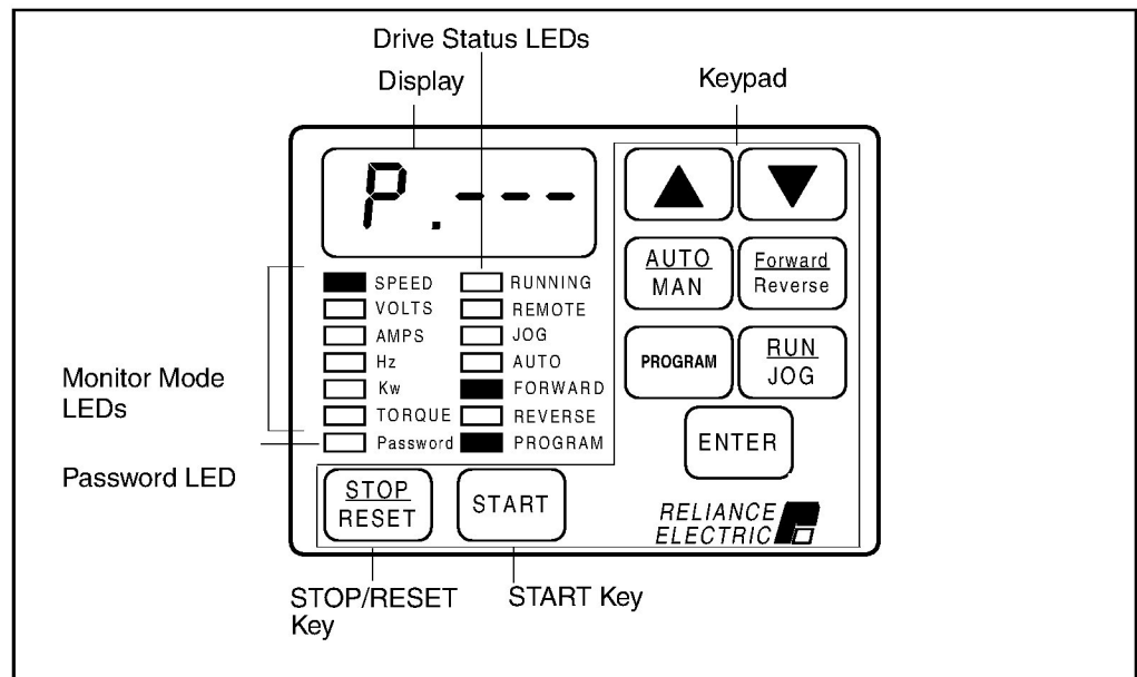
Figure 2.15 – Keypad/Display
