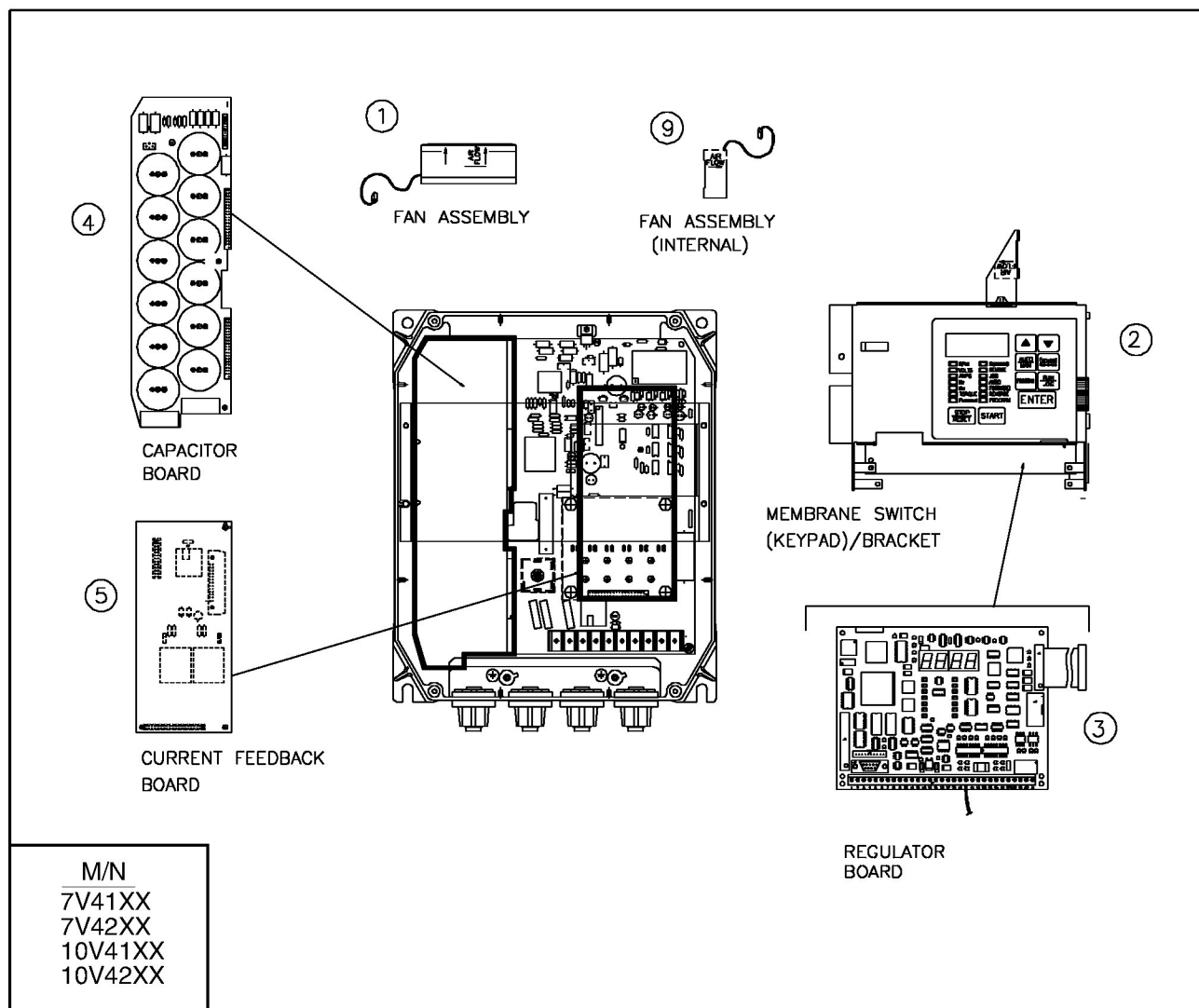
Figure 2.3 – 7.5-10 HP Drive Component Locations
