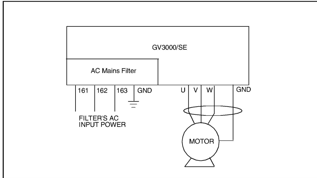
Figure C.6 – Typical Three-Phase Connections for Built-in AC Mains Filters in GV3000/SE Drives M/N 50T41xx and 75T41xx
