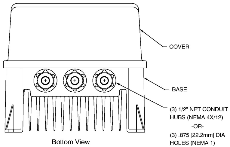
Figure 4.1 – Wire Routing Locations for 1-5 HP Drives
