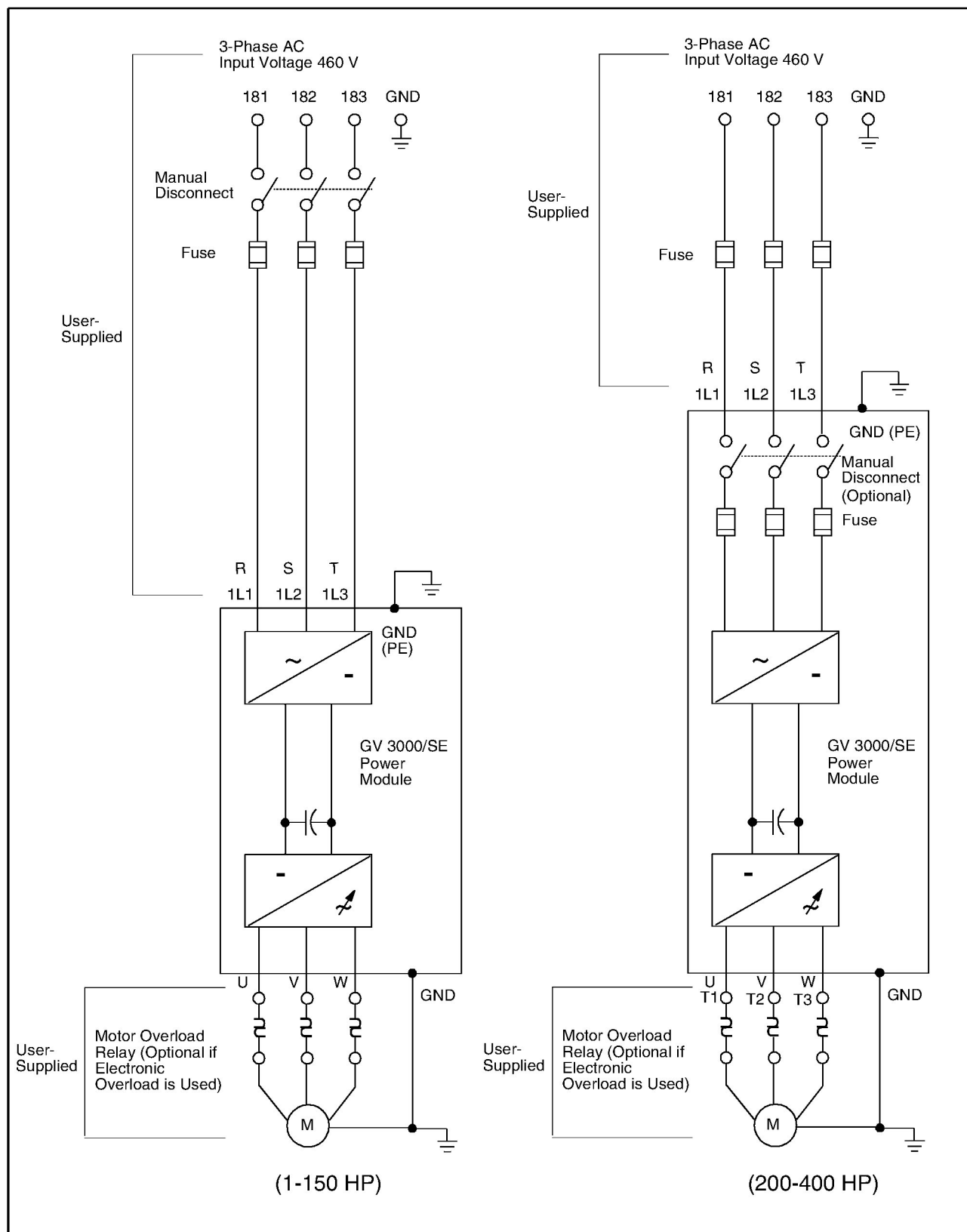
Figure 5.1 – Typical AC Input Electrical Connections
