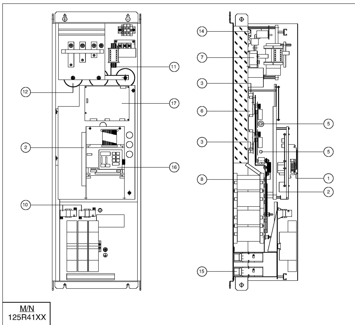
Figure 2.7 – 100-150 HP Drive Component Locations
