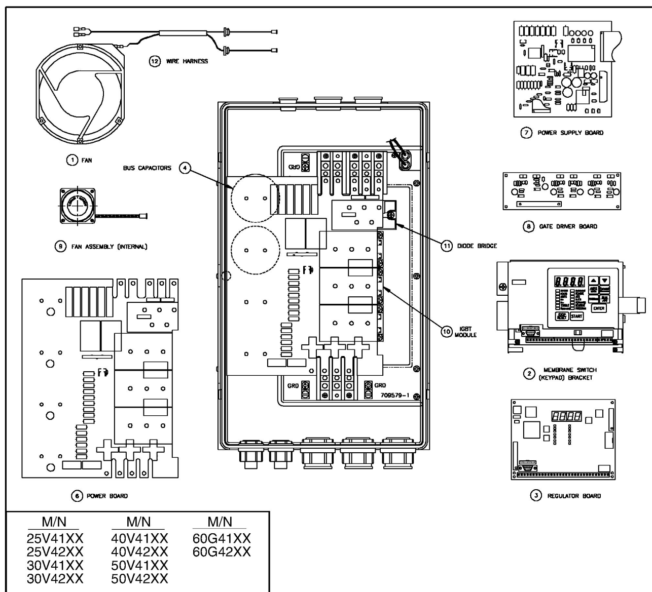
Figure 2.5 – 25-60 HP Drive Component Locations
