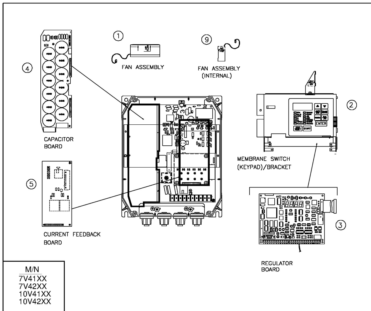
Figure 2.3 – 7.5-10 HP Drive Component Locations
