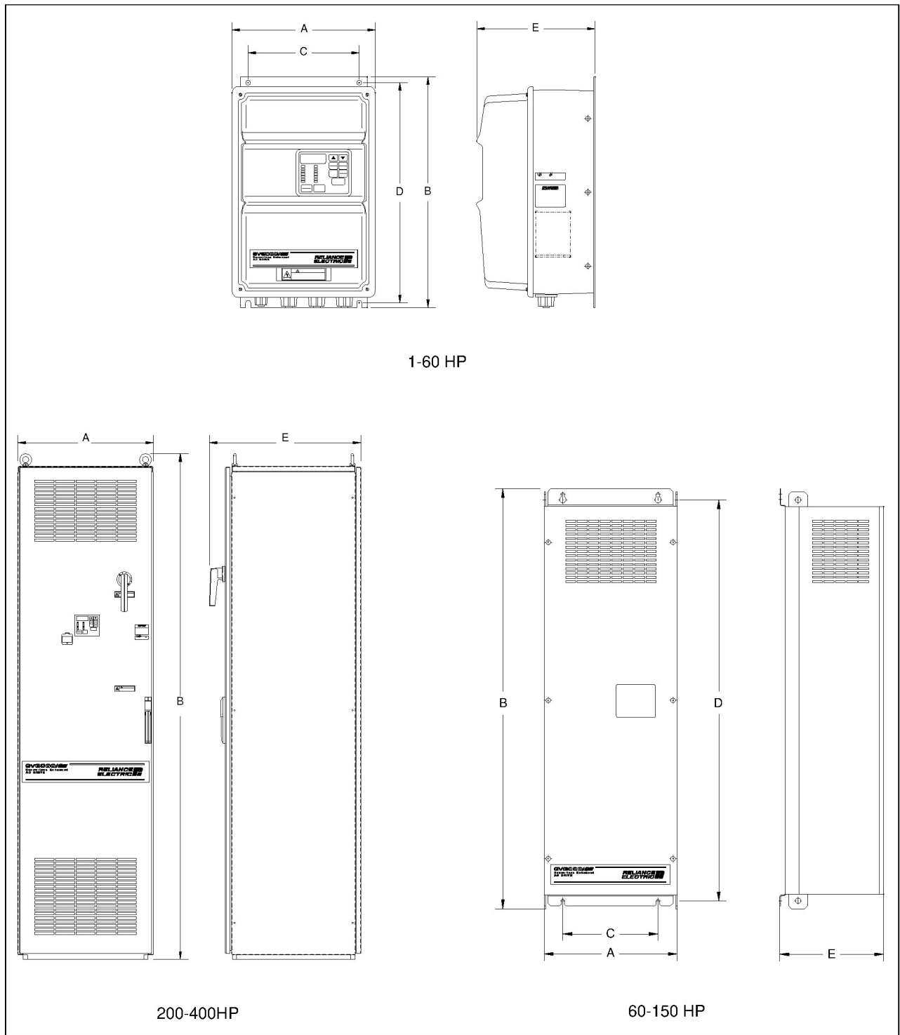
Figure 3.1 – Drive Dimensions
