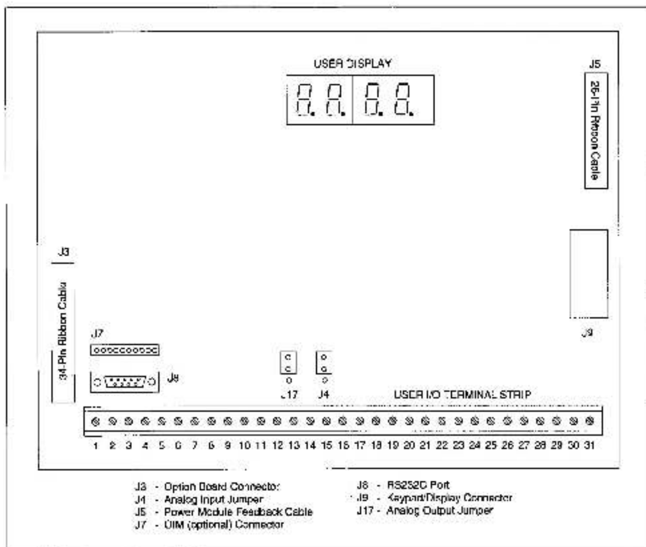
Figure 2.7 — Regulator Board Component Locations
