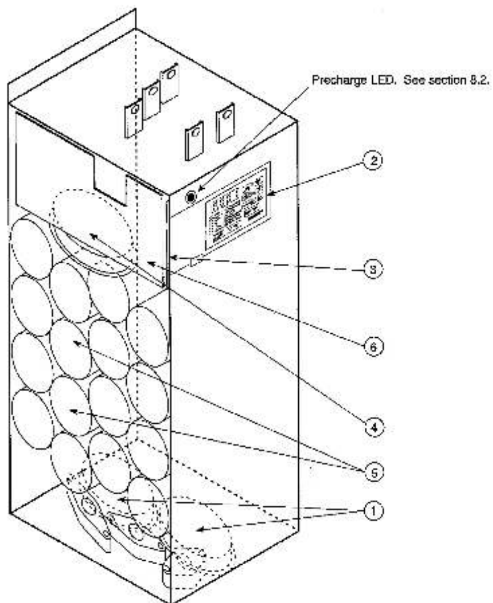
Figure 2.8 – 160 and 200 HP Drive Component Locations
