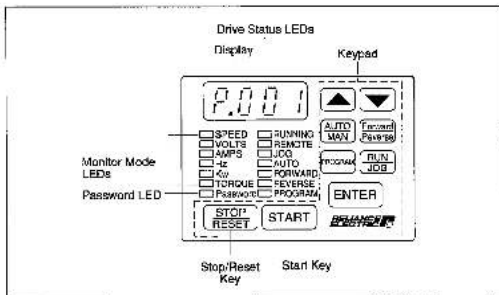
Figure 2.11 – Keypad/Display
