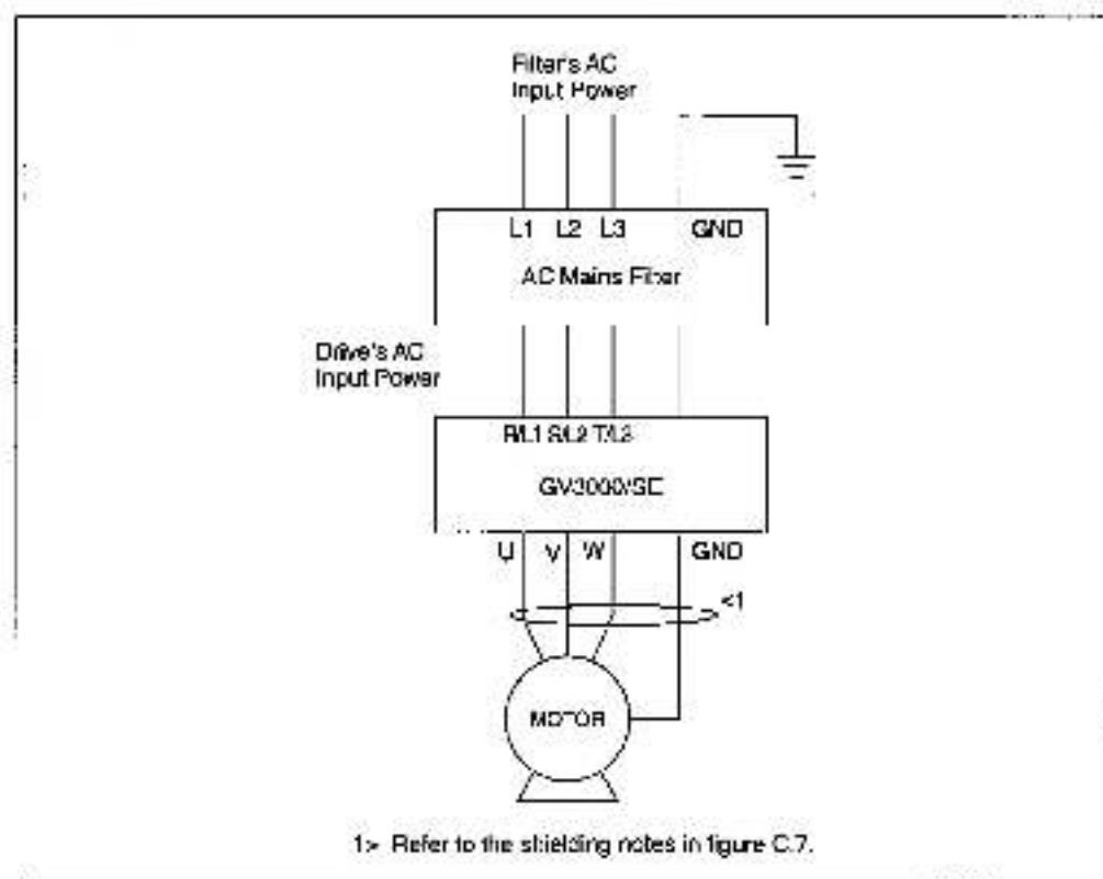
Figure C.8 - Typical Three-Phase Connections for AC Mains Filter
