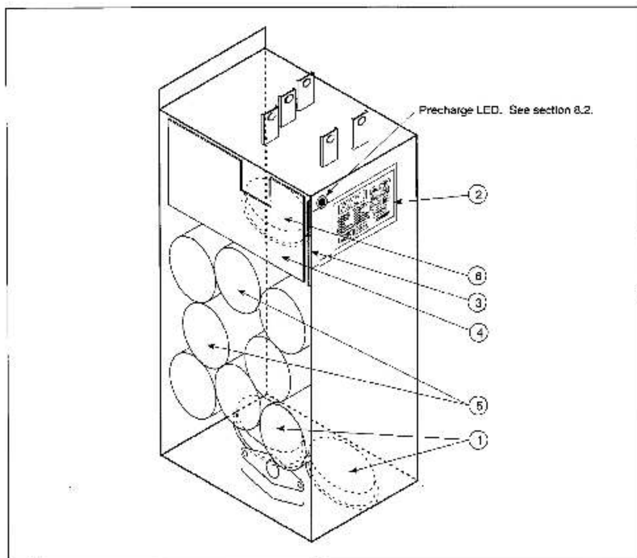
Figure 2.4 – 75 and 100 HP Drive Component Locations
