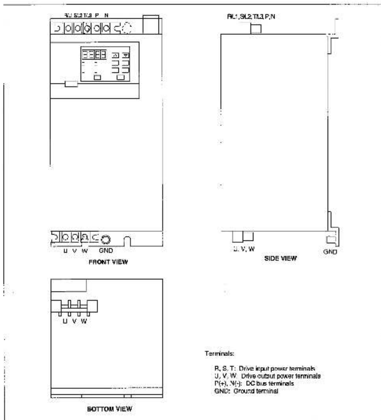
Figure 4.1 – Terminal Locations of 30 HP and 40 HP Drives
