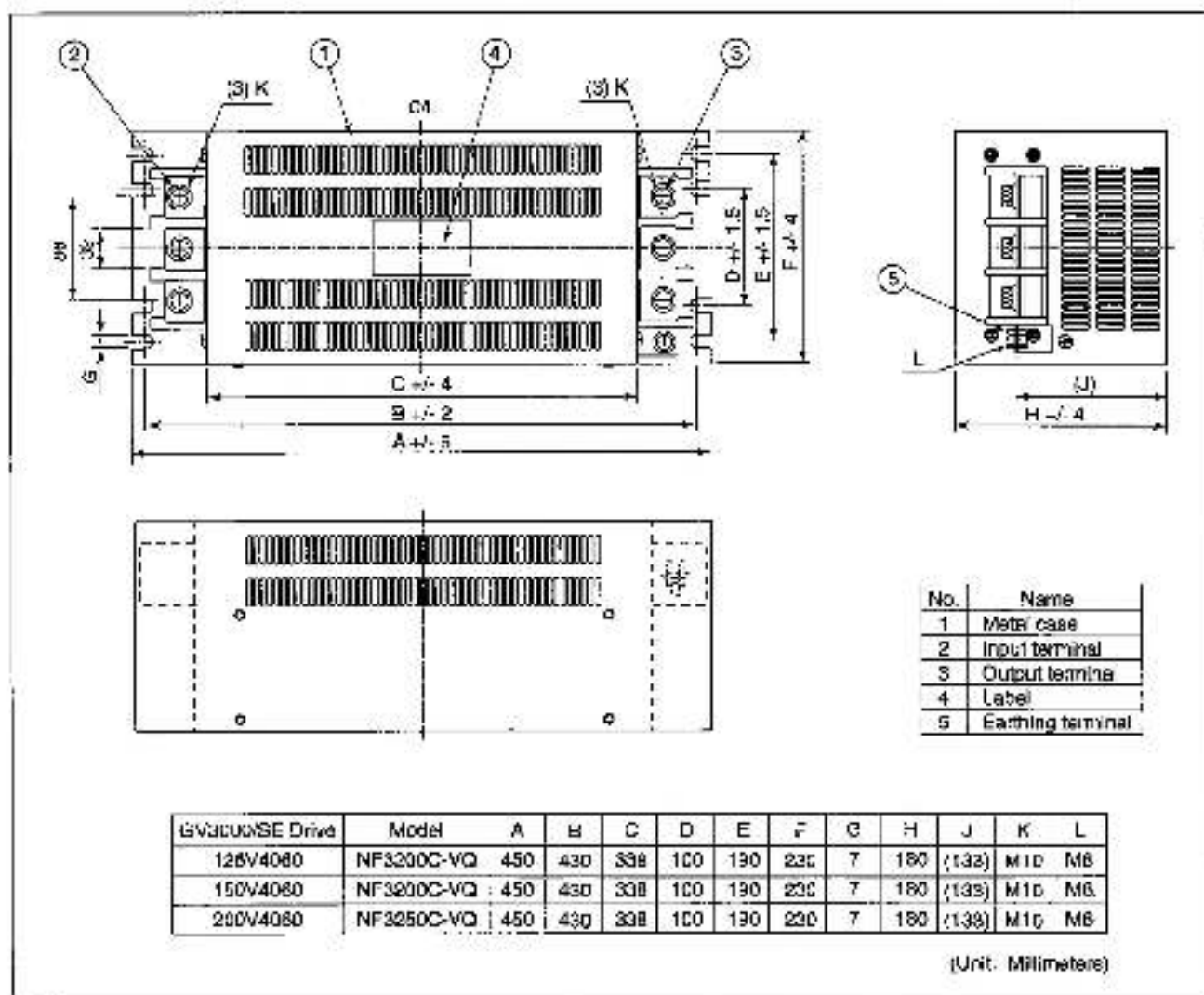
Figure C.4 - Outline Dimensions of AC Mains Filters of Sashin Electric for Model 125V4080 to 200V4080 Drives
