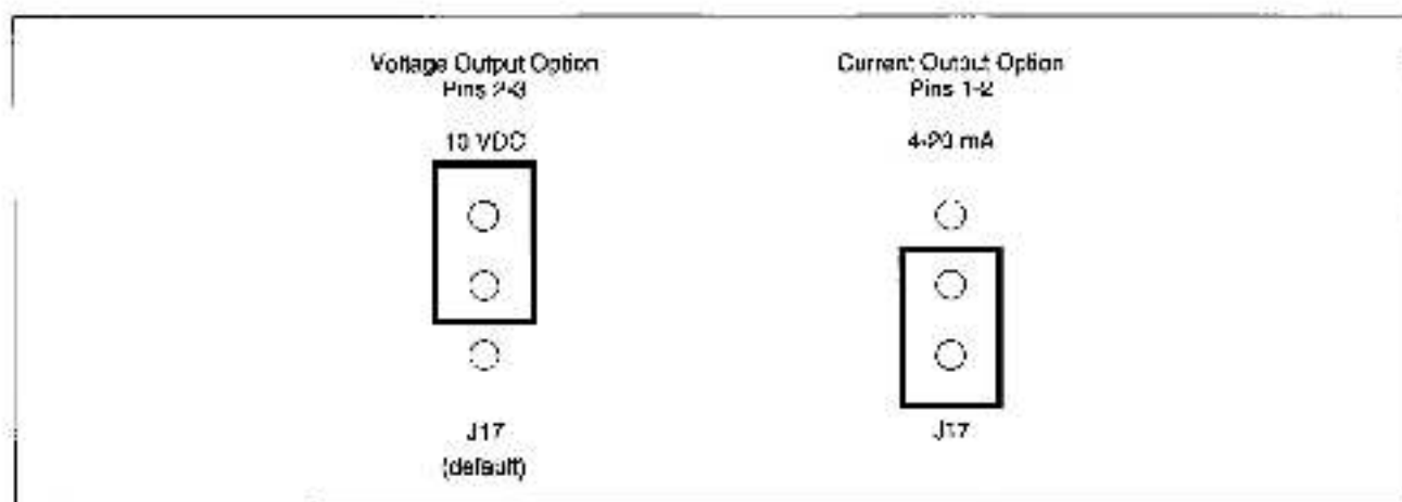
Figure 2.9 – Jumper J17 Settings for Analog Outputs
