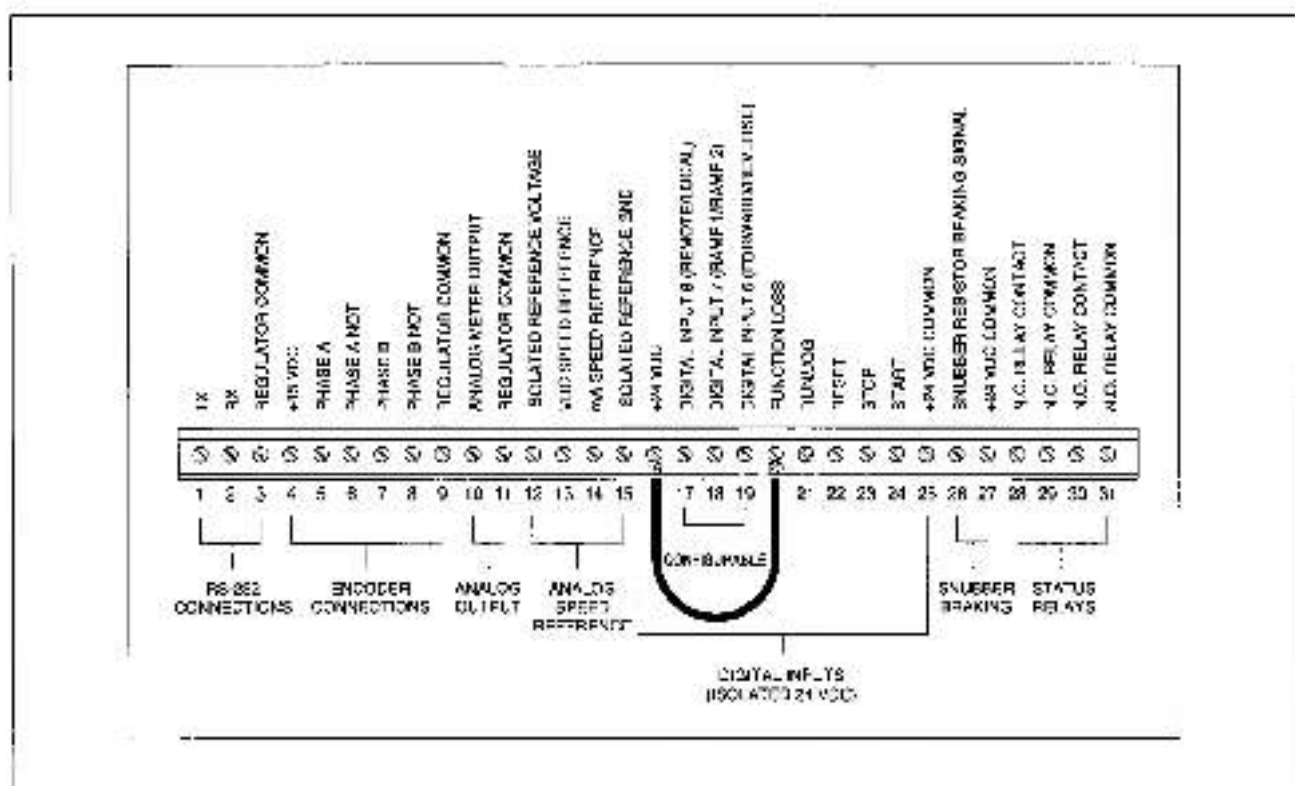
Figure 2.10 – Typical Terminal Strip Connections
