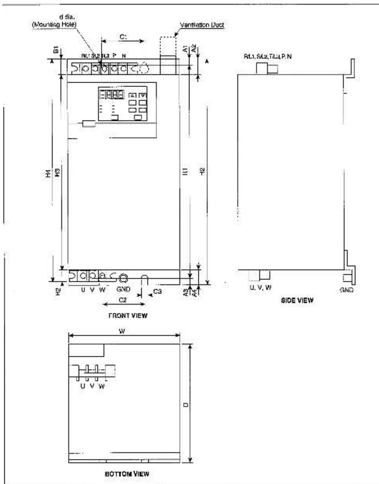
Figure 3.1 - Dimensions of 30 HP and 40 HP Drives
