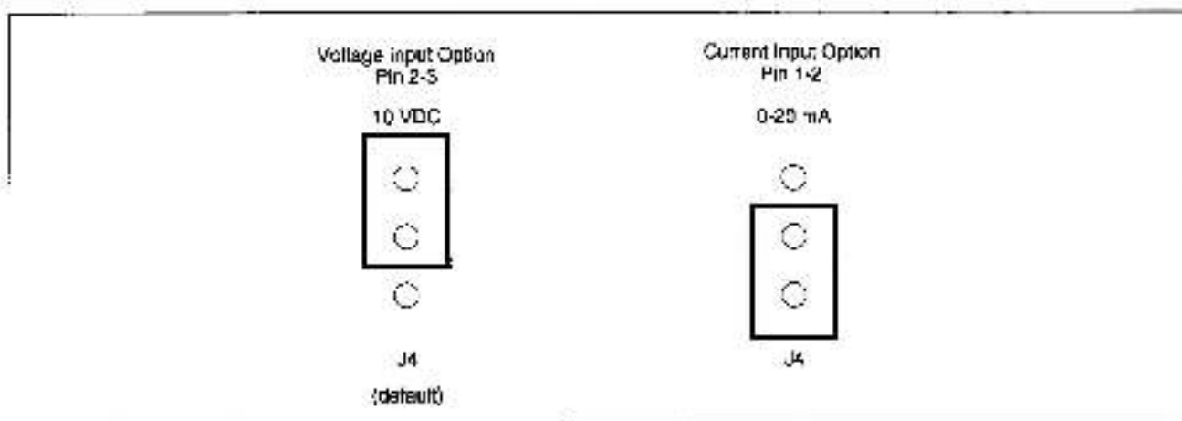
Figure 2.8 – Jumper J4 Settings for Analog Input Speed Reference
