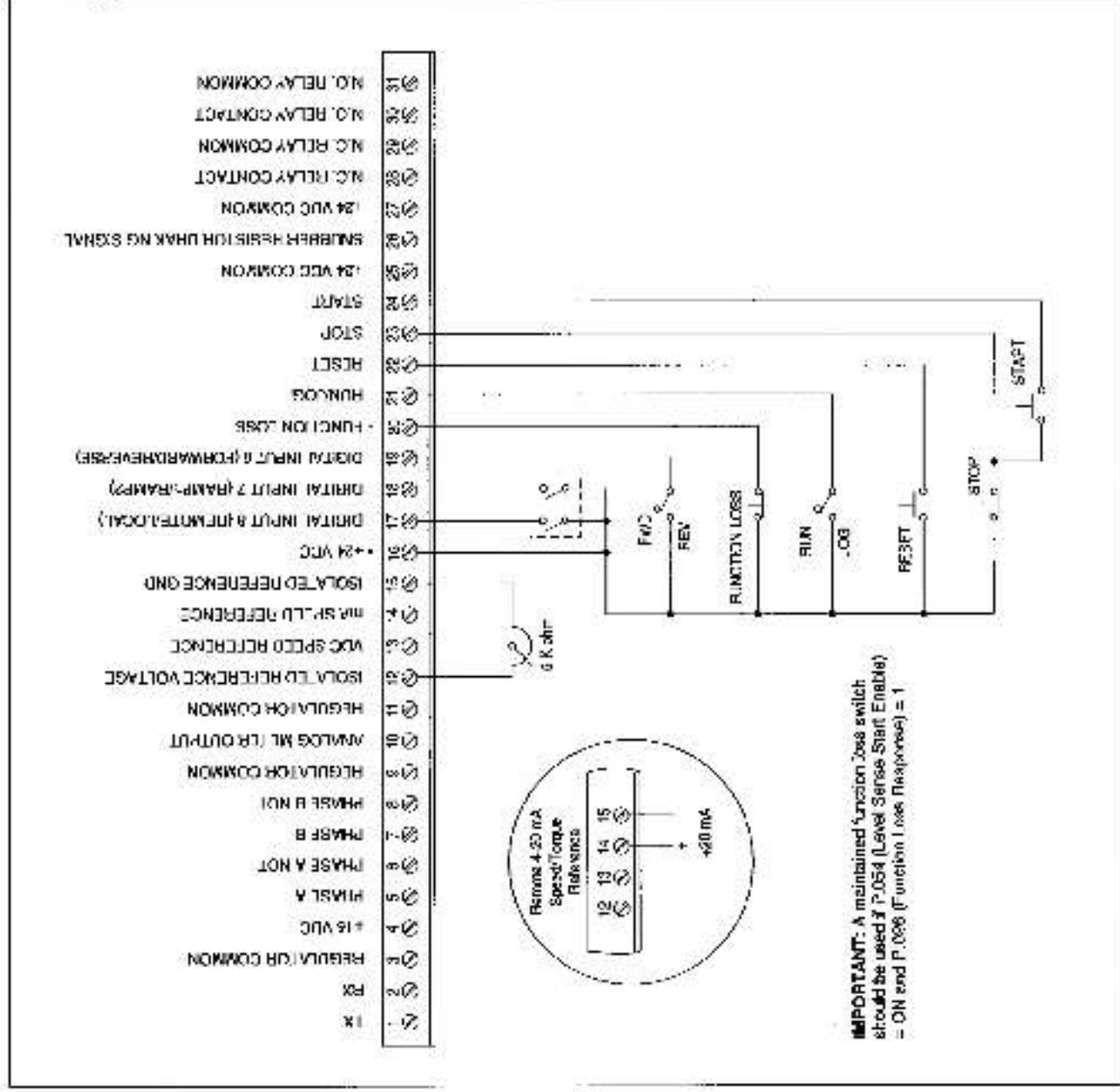
Figure 7.2 – Three-Wire Start/Stop Sample Control Wiring
