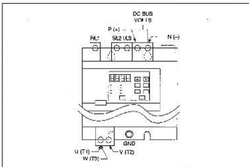
Figure 9.2 – DC Bus Voltage Terminals of 50 HP to 200 HP Drives
