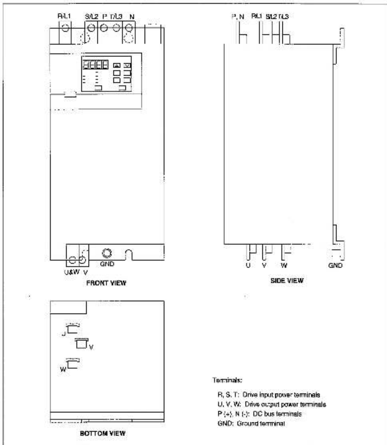
Figure 4.2 - Terminal Locations of 50 HP to 200 HP Drives
