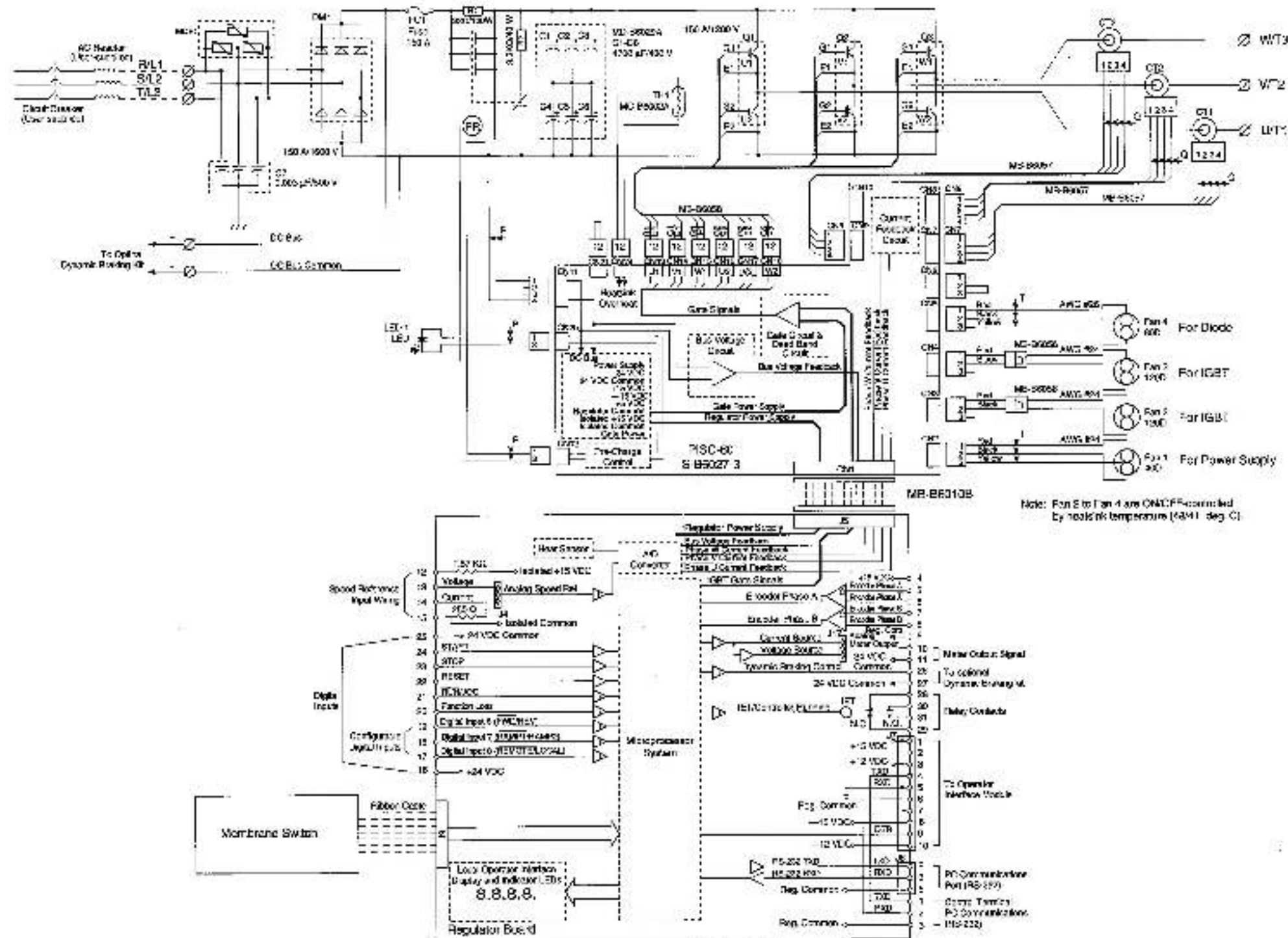
Figure B.2 - 50-60 HP GV3000/SE System Wiring Diagram
