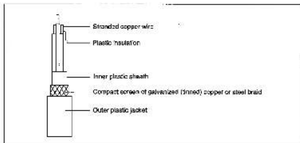
Figure C.9 - I/O Signal Cable
