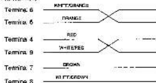
Figure 7-2 - Encoder Wiring Connections
