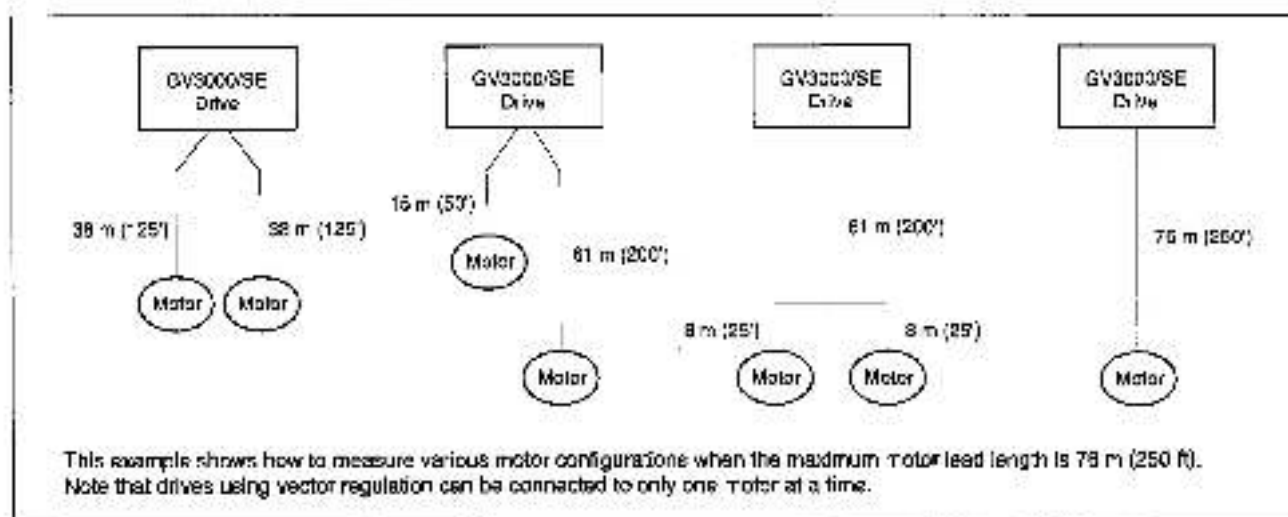
Figure 3.4 — How to Calculate Motor Lead Lengths
