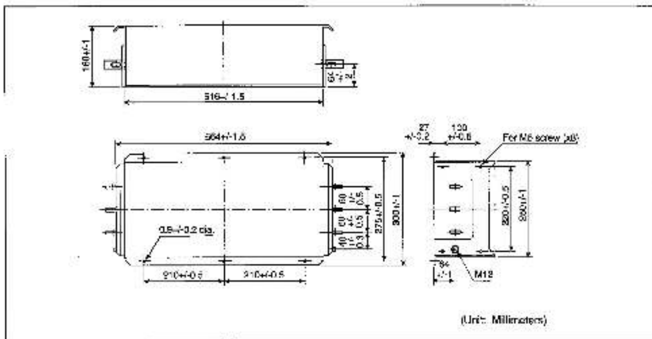
Figure C.2 - Outline Dimensions of Model FN350H250/30 AC Main Frame of Schaffner for Model 150V4060 and 200V4060 Drives
