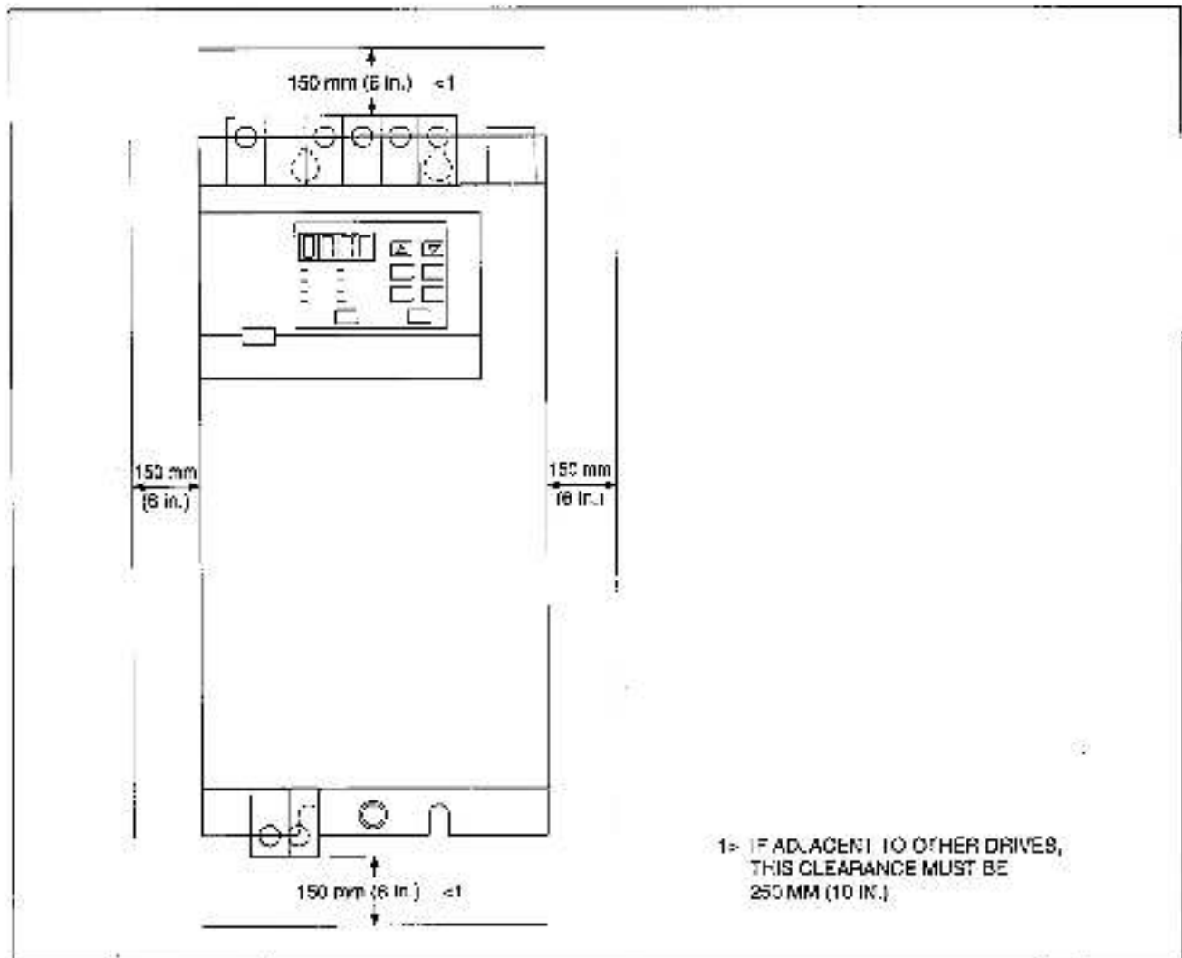
Figure 3.3 – Recommended Air Flow Clearances
