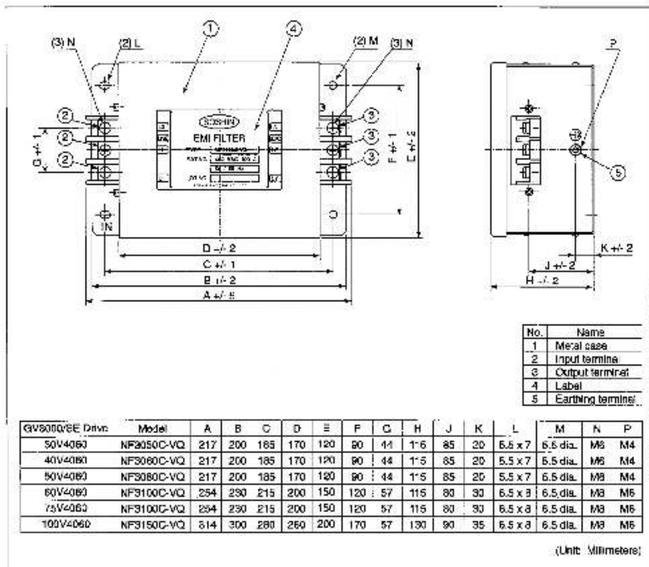
Figure C.3 - Outline Dimensions of AC Mains Filters of Soshin Electric for Model 30V4060 to 100V4080 Drives
