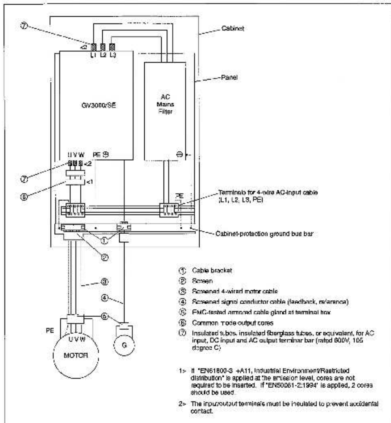
Figure C.7 - Cabinet Mounted GV3000/SE Wiring Example
