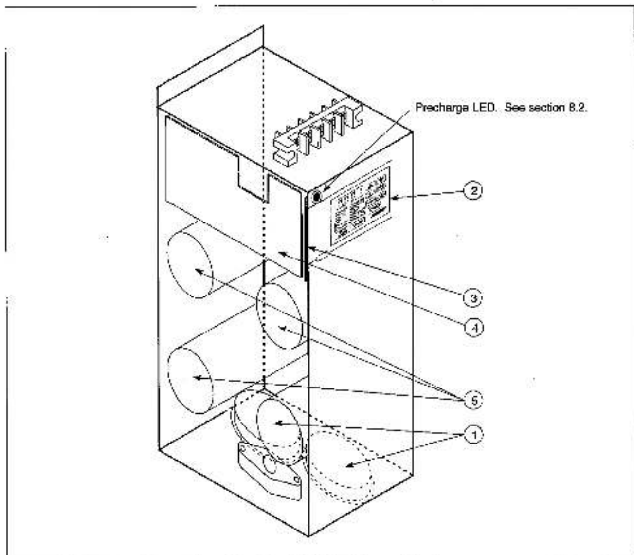
Figure 2.2 - 30 and 40 HP Drive Component Locations
