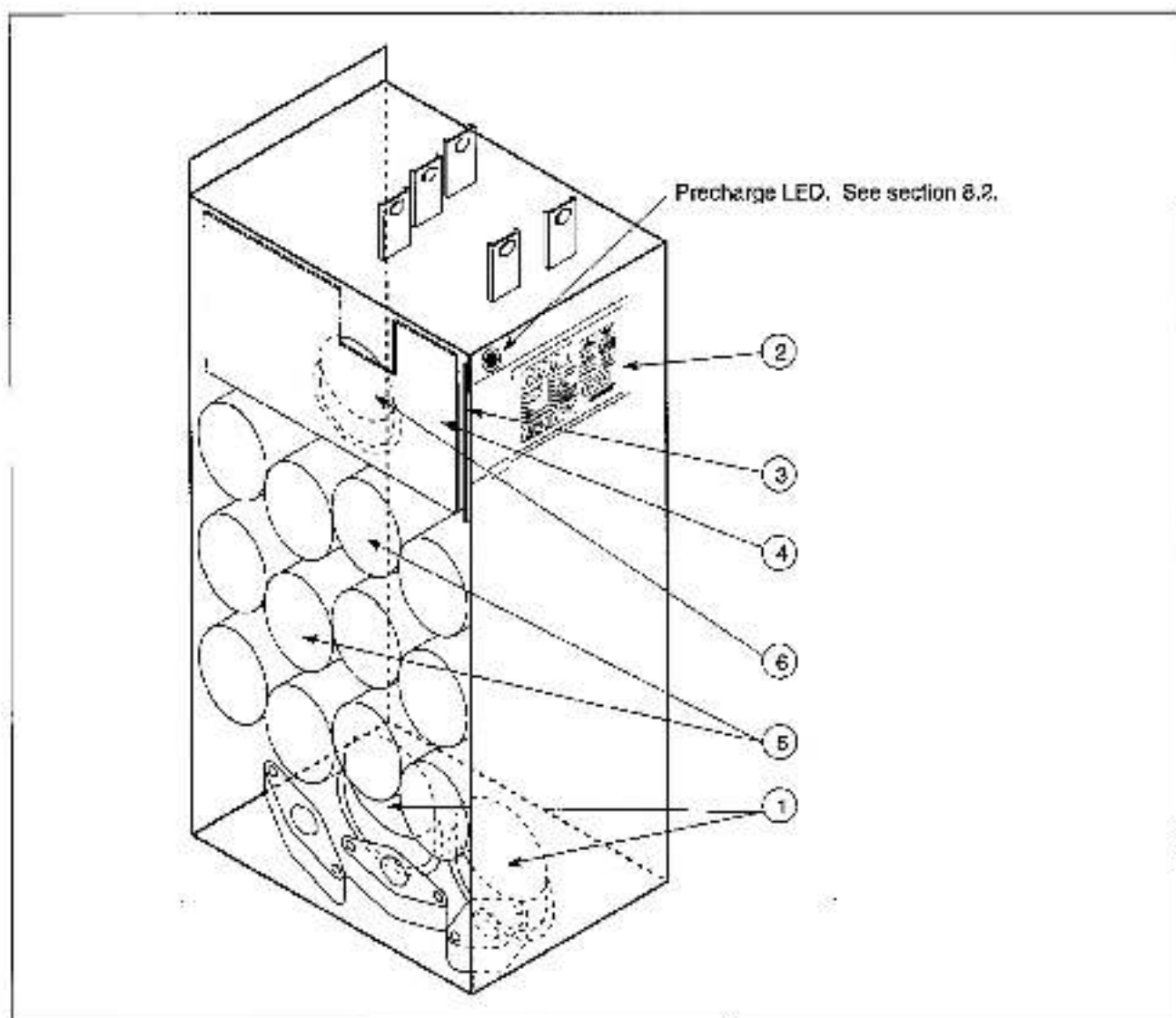
Figure 2.5 – 125 HP Drive Component Locations
