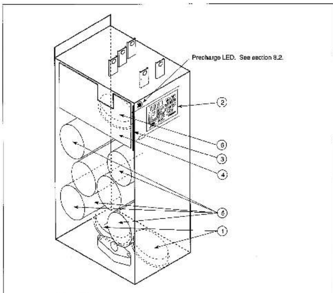
Figure 2.3 – 50 and 60 HP Drive Component Locations
