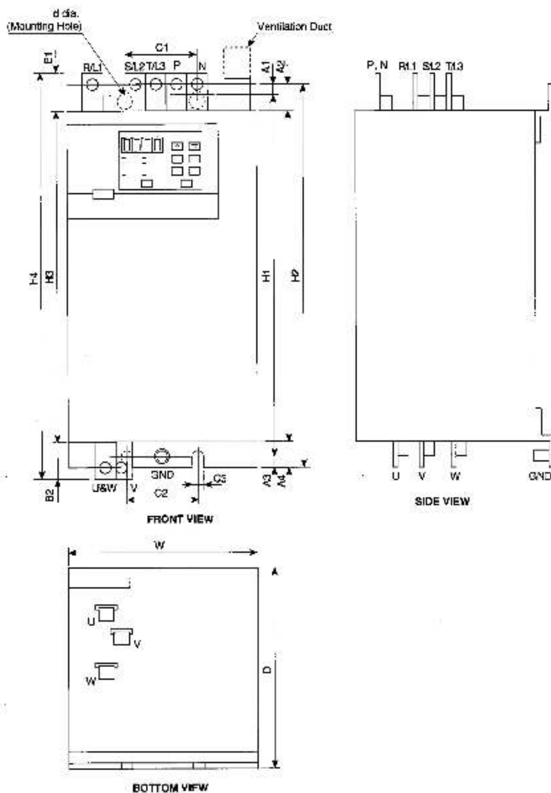
Figure 3.2 – Dimensions of 50 HP to 200 HP Drives
