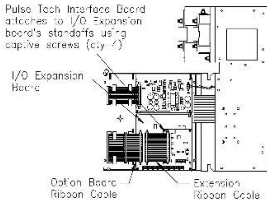
Figure 6 - Installing the I/O Expansion Board (with Pulse Tach Board)
