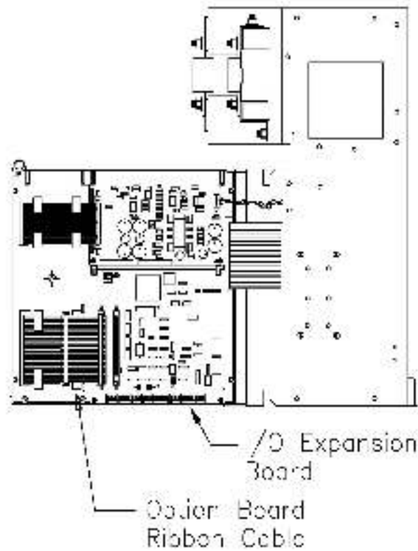
Figure 5 - Installing the I/O Expansion Board (w/o Pulse Tach Board)
