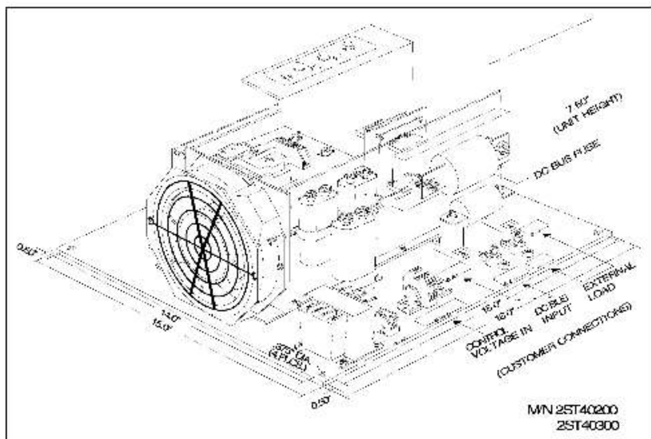
Figure 6 Transistor Braking Module Dimensions - Style F (Open Enclosure)
