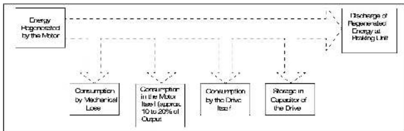
Figure 1 — Dissipation of Energy Regenerated by the Motor
