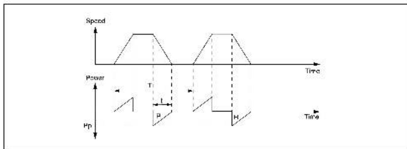
Figure 6 – An Example of Repeated Operation Under Inertial Load
